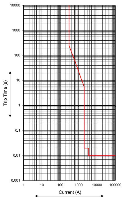
DN2T MTX2.0
