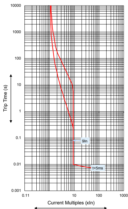
DN0 MCCB
