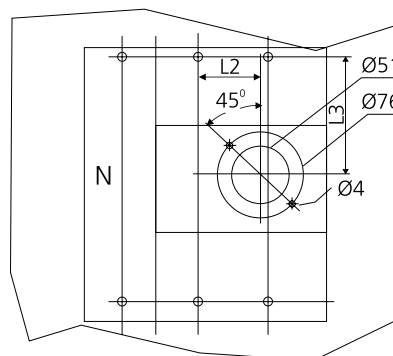
Mounting & Door Cut-out Details
